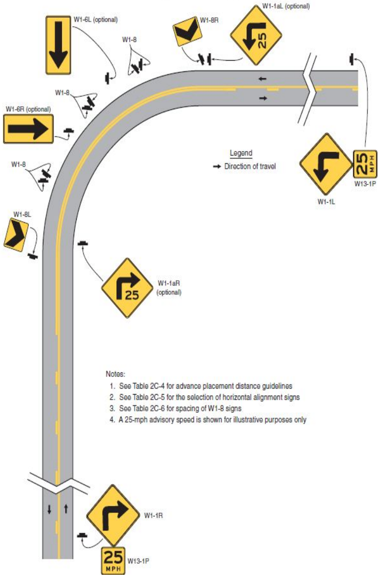
Figure 2C-2. Example of Warning Signs for a Turn
