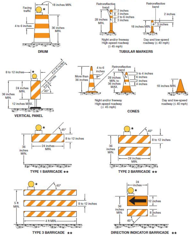
Figure 6F-7. Channelizing Devices
