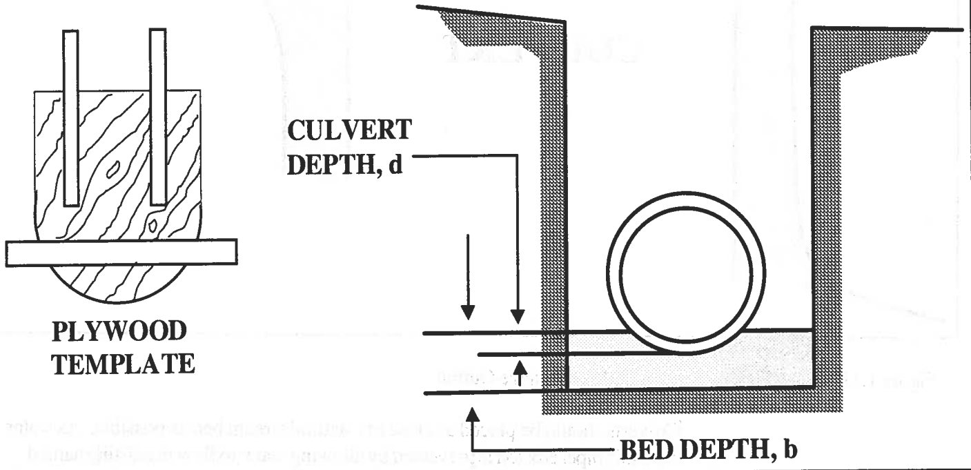
Figure 1.12 - Culvert Bedding
