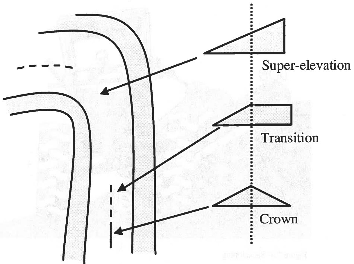
Figure 3.5-Super-elevation on Curves
